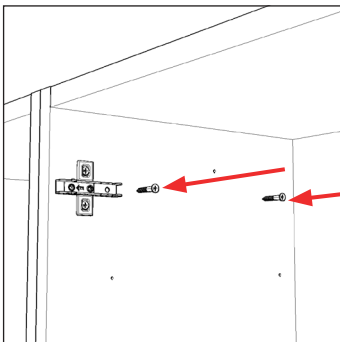
Detail A Secure to adjacent cabinet top
