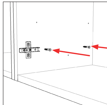
Detail B Secure to adjacent cabinet bottom
